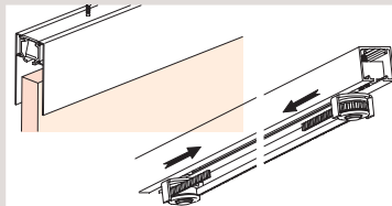
SF-SINCRO FITTING SET X2 SOFTBRAKE
